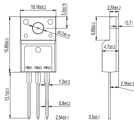
ITO-220AB MURA20XXFCT MURL20XXFCT MURR20XXFCT
