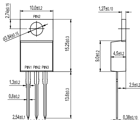
TO-220AB MURA20XXCT MURL20XXCT MURR20XXCT
